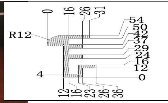
Shutter frames
