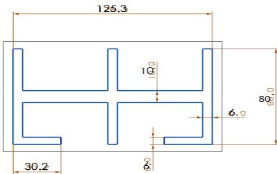
王-shaped profile
