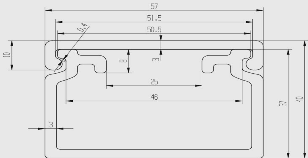
Special channel
